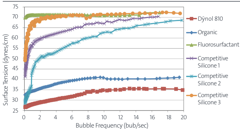
Figure 1: Dynamic surface tension 0.1 wt % surfactant in water
