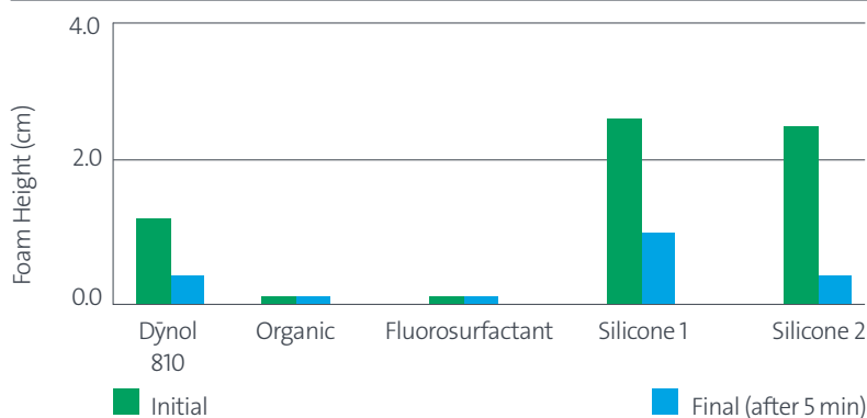
Figure 2: Ross-Miles foam
